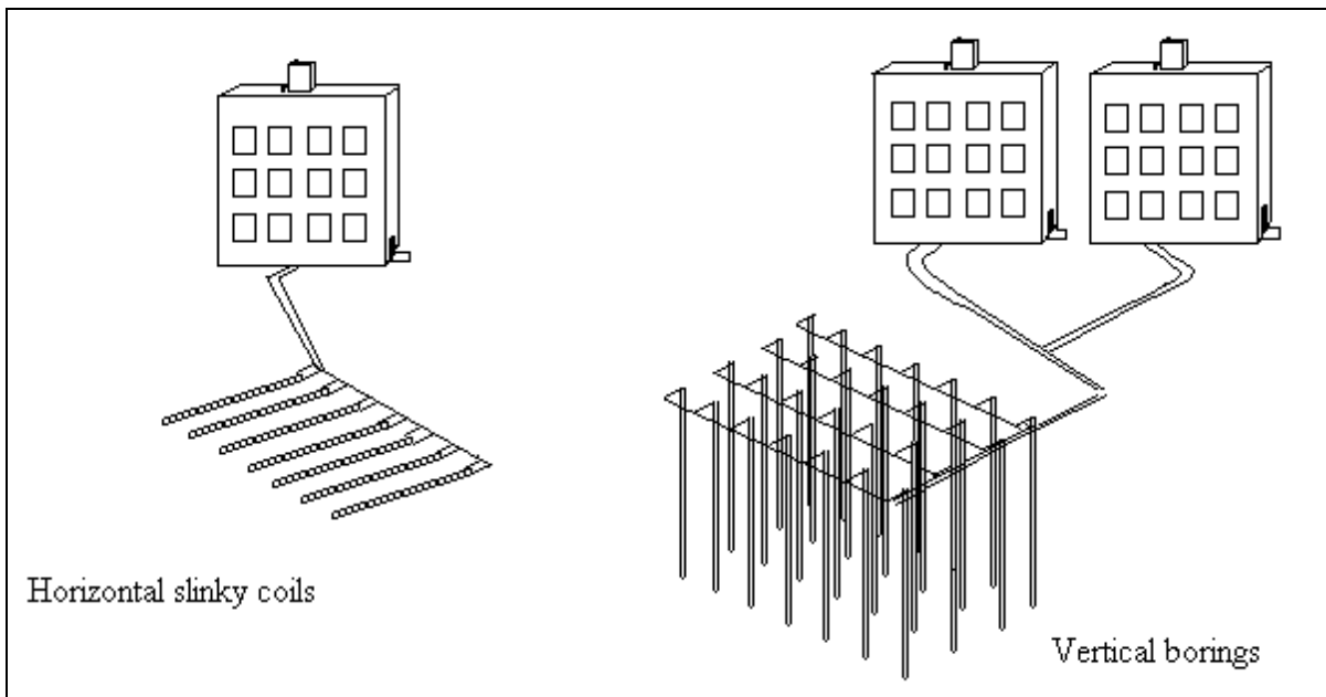
FIGURE 4. COMMERCIAL GSHP SYSTEMS (not to scale)
