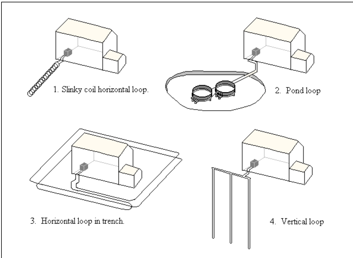
FIGURE 2. SERIES LOOP CONFIGURATIONS (not to scale)
